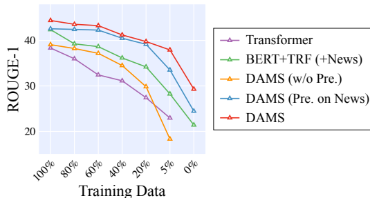
Figure 2: Model performance in low-resource settings.
