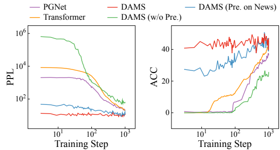
Figure 3: Fine-tuning logs of different models on the SAMSum dataset. PPL and ACC represent perplexity and word accuracy, respectively.
