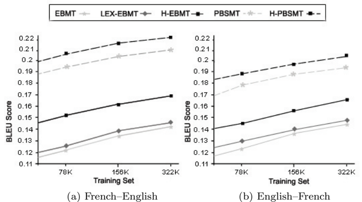
Figure 1: BLEU scores for various baseline and hybrid EBMT and PBSMT systems, for French–English and English–French
