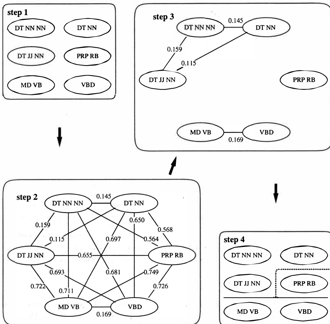
Figure 2: Clustering part-of-speech sequences ( D_{min} = 0.25 )
