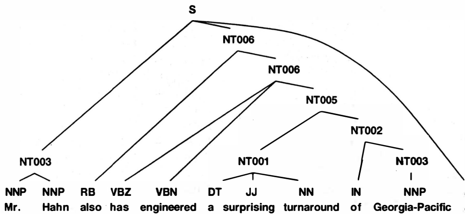
Figure 4: An example of a parsed sentence (Exp. 2)
