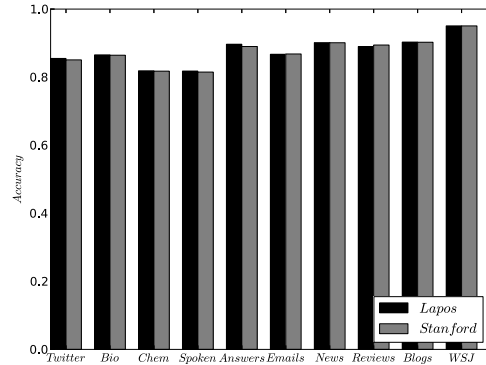
Figure 1: Accuracies of LAPOS vs. STANFORD across 10 data sets.
