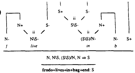
Figure 5: Proof-net for 'Frodo lives in Bag End'
