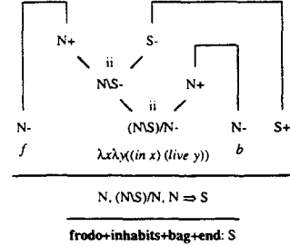
Figure 6: Proof-net for 'Frodo inhabits Bag End'
