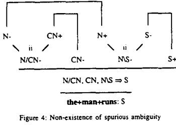
Figure 4: Non-existence of spurious ambiguity
