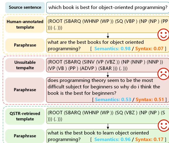
Figure 1: The generated paraphrases with different templates. “Semantics” and “Syntax” represent the semantic similarity with the source sentence and the syntactic distances against the template, respectively. Obviously, an unsuitable template may lead to a poor paraphrase.
