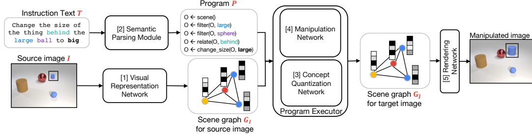
Figure 3: High level architecture of NEUROSIM. See Section 3 for more details.
