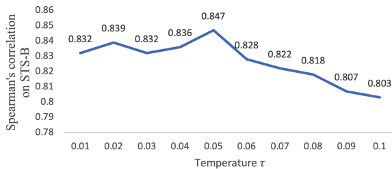
Figure 5: Effect of the temperature \tau in ArcCon loss. Results are reported on the development set of STS-B based on the Spearman's correlation.
