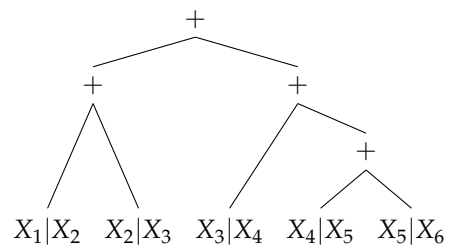
(b) Separating tree for canonical linearization.
