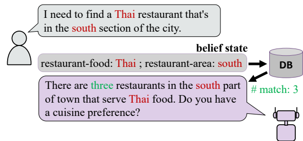
Figure 1: The cues for inferring belief states from user inputs and system responses. The system response reveals the belief state either directly in the form of word repetition (red), or indirectly in the form of the database query result (green) determined by the belief state.
