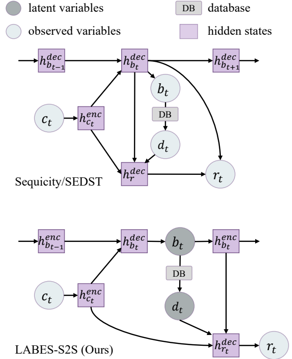
Figure 5: Comparison of computational graphs.
