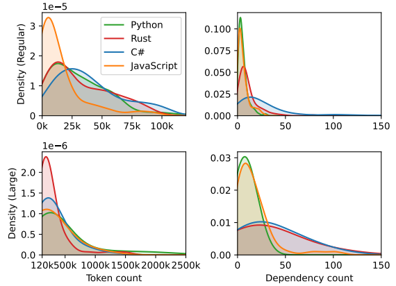
Figure 10: Distribution of token and dependency count.
