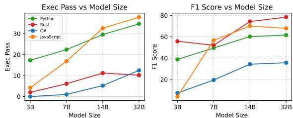
Figure 12: Model performance across programming languages for Qwen2.5-Coder-Instruct
