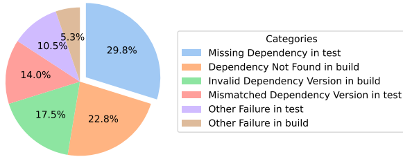
Figure 4: Distribution of failure categories (GPT-4o, All-In-One setting, Python).
