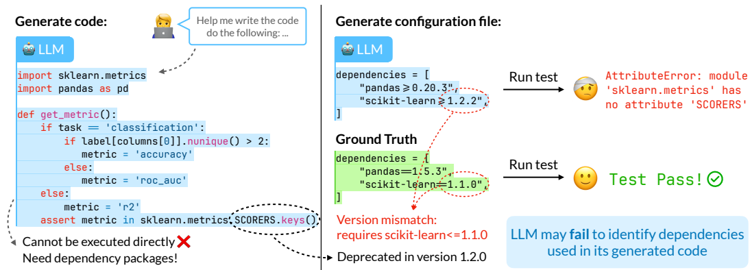
Figure 2: An example of incorrectly identifying dependencies used in code.
