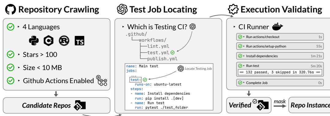
Figure 3: CI-based curation pipeline for DI-BENCH.
