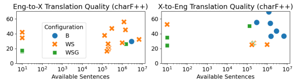
Figure 1: Using grammars is particularly beneficial for extremely low-resource languages. Simple prompt-based MT (zero-shot) is best for high-resource ones.
