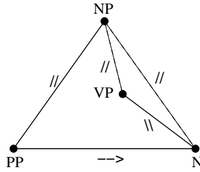
Figure 5: Scoping induced cycles: NP \{ // PP \rightarrow N \setminus \setminus VP \}
