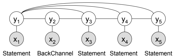
Figure 1: A skip-chain CRF with pragmatic-level links.
