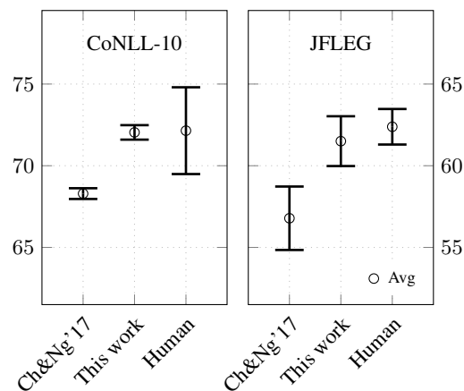
Figure 3: Comparison with human annotators. The figure presents average M 2 and GLEU scores with standard deviations.
