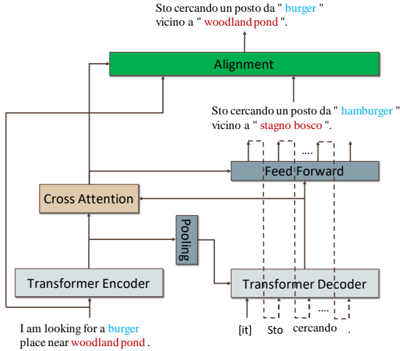
Figure 2: Example of the translation and alignment process. The encoder-decoder cross-attention weights are used to achieve word alignment.
