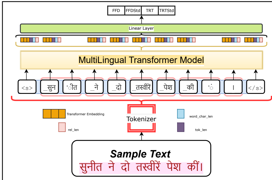
Figure 1: Model Representation
