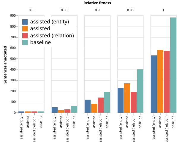
Figure 4: Minimum number of sentences necessary to reach a specific performance relative to the target F_1 with each active learning strategy for sentence suggestion.
