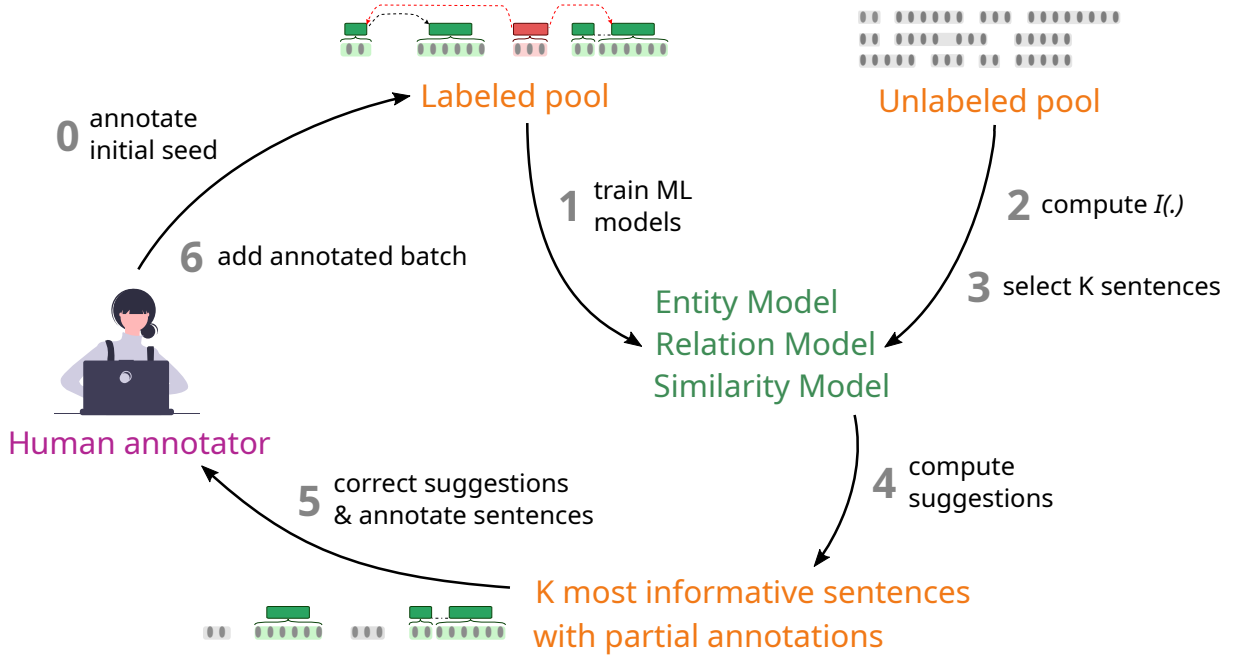
Figure 1: High-level illustration of the active learning strategy presented in this research for human-in-the-loop annotation of entity-relation corpora.
