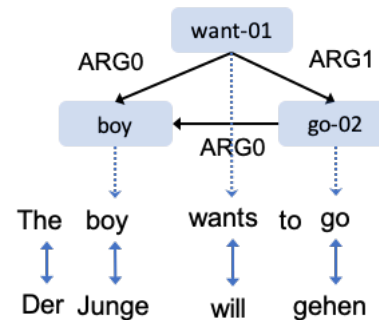
Figure 1: AMR graph for The boy wants to go and its German translation Der Junge will gehen . Implicit alignments between the English text and AMR concepts are denoted by dotted arrows. Explicit alignments between English and German texts are denoted by solid arrows.
