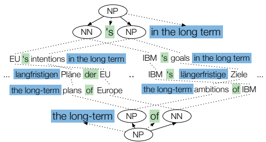
Figure 2: Extraction of syntactic paraphrases via the pivoting approach: We aggregate over different surface realizations, matching the lexicalized portions of the rule and generalizing over the nonterminals.
