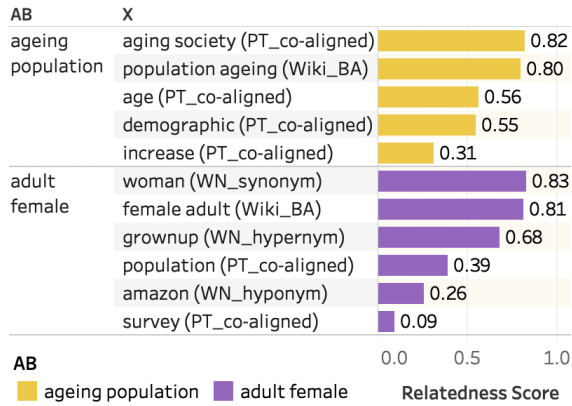
Figure 1: Example entries from BiRD.
