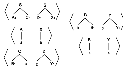
Figure 2: An example of synchronous CFG
