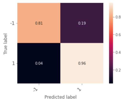
Figure 3: Confusion matrix for Experiment 4 with SrpELTeC-2C
