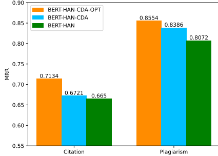
Figure 4: Plausibility comparison among BERT-HAN, BERT-HAN-CDA and BERT-HAN-CDA-OPT ( hard ) on S2ORC (Citation) and PAN (Plagiarism).
