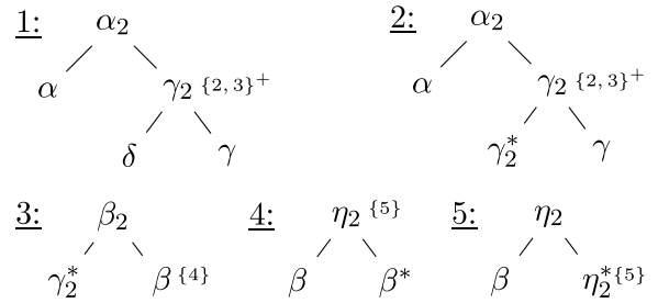
Figure 4: Tree-adjoining grammar.
