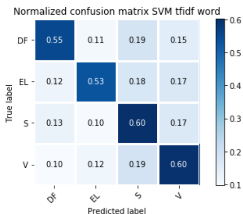
Figure 1: Confusion matrix
