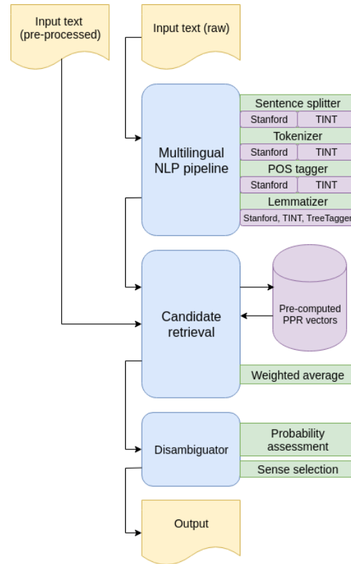
Figure 1: Architecture diagram of SyntagRank.
