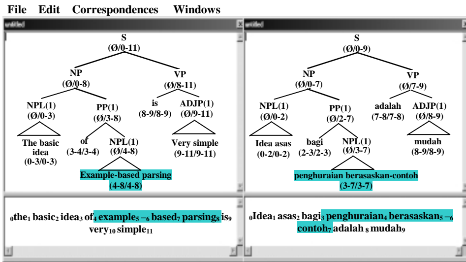
Figure 6: The synchronous SSTC editor.
