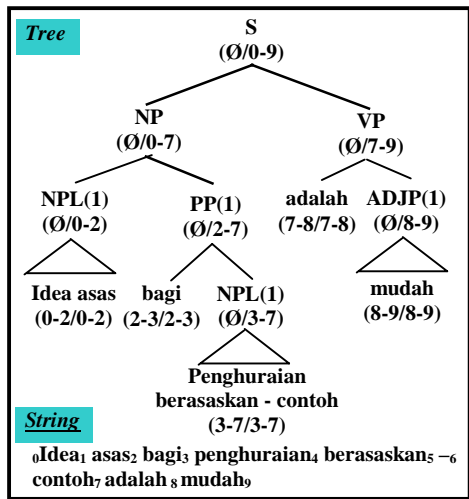
Figure 4: An SSTC construction for the Malay sentence “ idea asas bagi penghuraian berasaskan-contoh adalah mudah ” after lexical transfer.
