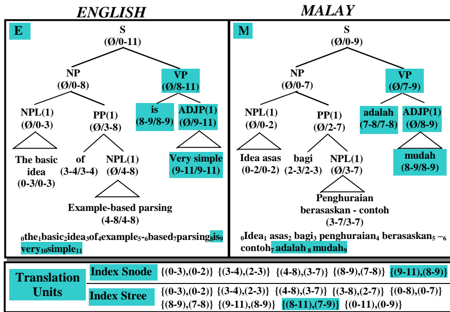
Figure 5: Example synchronous SSTC for the English sentence “ the basic idea of example-based parsing is very simple ” and the Malay sentence “ idea asas bagi penghuraian berasaskan-contoh adalah mudah ” together with their translation units.
