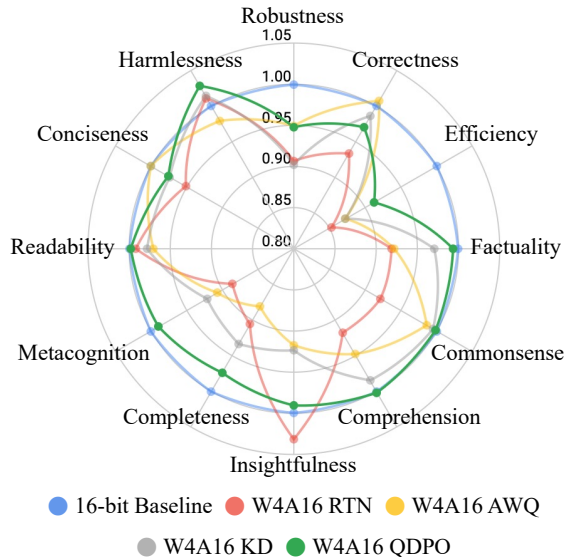
Figure 6: Performance relative to baseline on FLASK. Absolute performance results can be found in Table 9.
