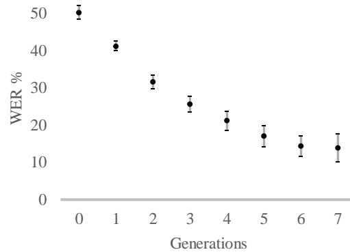
Figure 1. ASR results trained on SHARPened lexical-phonetic forms. The graph shows Word-error rates (WER) for each SHARP generation. Error bars: standard deviation for data sets after ten-fold cross validation. Average WER keeps improving somewhat in generations >7, however less significantly so as error margins increase.
