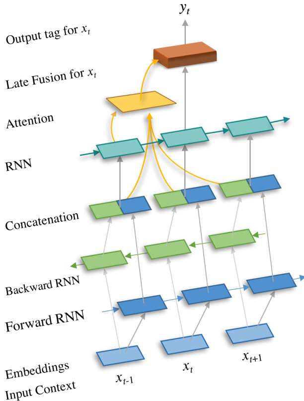
Figure 1: Neural network design for punctuation restoration. The diagram shows an input context for the word x_t and the stack of layers that result in the tag y_t representing the punctuation decision for x_t .
