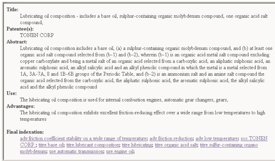
Figure 2: Example of a patent abstract with its generated multi-index. The multi-index that has been generated for the above patent abstract corresponds to the “ Final indexation ” field. The terms of the generated multi-index are prefixed by the name of the viewpoint to which they are associated: “adv.” for the Advantages viewpoint, “titre.” for the Title viewpoint, “use.” for the Use viewpoint, “soc.” for the Patentees viewpoint.
