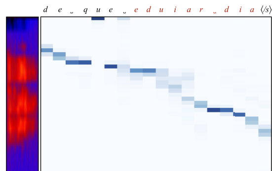
Figure 8: ASR attentions after regular decoding.
