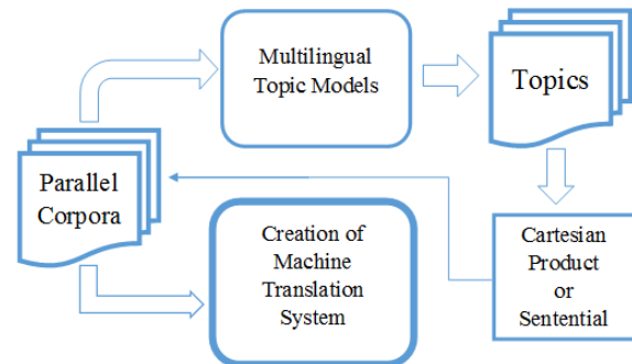
Figure 4: Our Architecture
