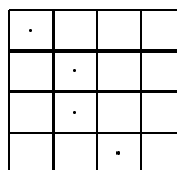
Figure 4: Global alignment
