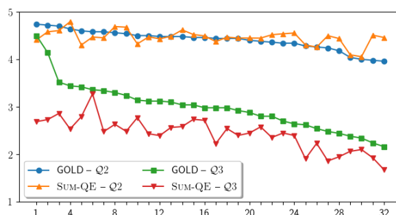
Figure 3: Comparison of the mean gold scores assigned for Q2 and Q3 to each of the 32 systems in the DUC-05 dataset, and the corresponding scores predicted by SUM-QE. Scores range from 1 to 5. The systems are sorted in descending order according to the gold scores. SUM-QE makes more accurate predictions for Q2 than for Q3 , but struggles to put the systems in the correct order.
