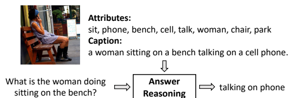
Figure 1: An example of explanation and reasoning in VQA. We first extract attributes in the image such as “sit”, “phone” and “woman.” A caption is also generated to encode the relationship between these attributes, e.g. “woman sitting on a bench.” Then a reasoning module uses these explanations to predict an answer “talking on phone.”
