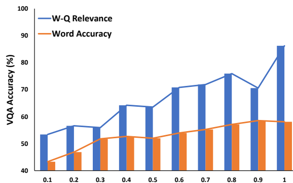
Figure 4: The comparison of the impact of word accuracy and word-question relevance on VQA performance.
