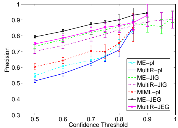
Figure 5: The precisions of different models under different confidence thresholds. The error bars represents the standard deviations of the results.
