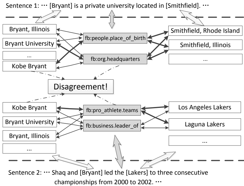
Figure 2: An example of our joint inference framework. The top and bottom are two example sentences with entity mentions in the square brackets, candidate entities in the white boxes, candidate relations in the grey boxes, and the solid lines with arrows between relations and entities represent their preference scores, with thickness indicating the preferences' value.
