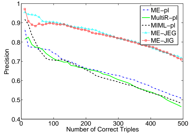
Figure 3: The numbers of correct triples v.s. the precisions for different approaches.
