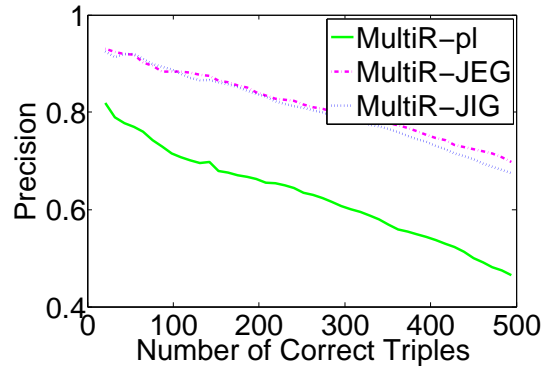
Figure 4: The numbers of correct triples v.s. the precisions for approaches with MultiR extractor.
