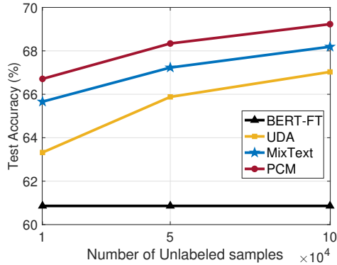
Figure 3: Accuracy on varying number of unlabeled data.
