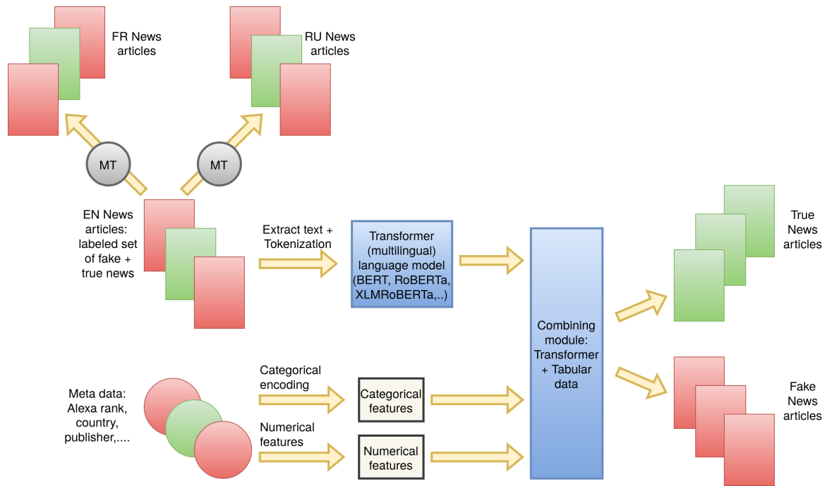
Figure 3: Supervised approach to fake news detection
