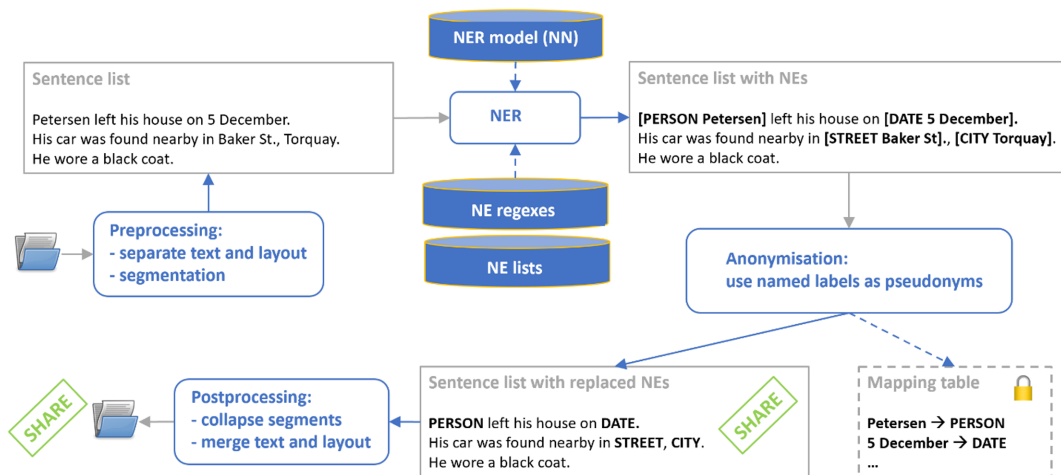
Figure 1: Scenario for workflow using NE labels
