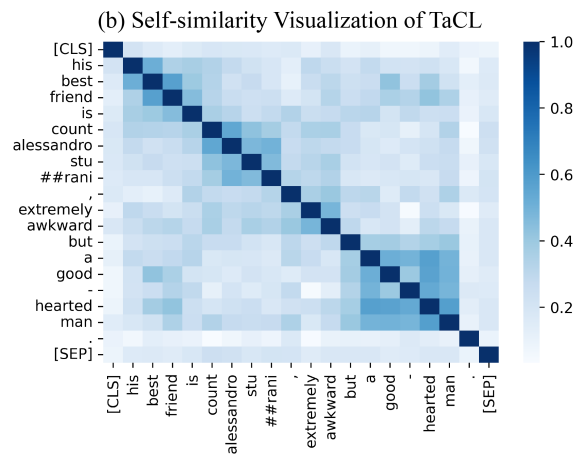
Figure 5: Example 3: self-similarity matrix visualization of (a) BERT and (b) TaCL. (best viewed in color)
