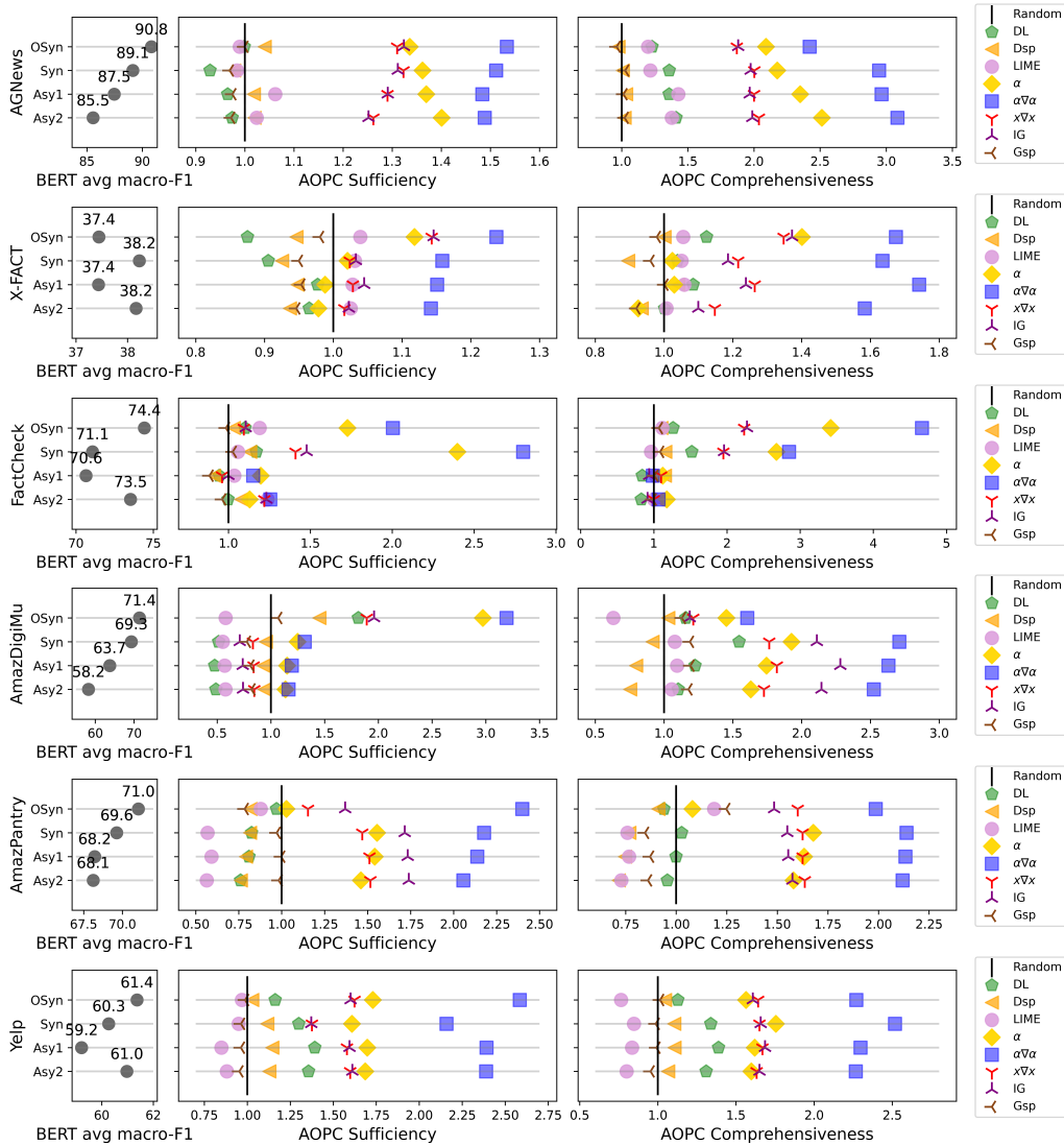
Figure 2: Post-hoc AOPC normalized sufficiency and comprehensiveness (higher is better) of the original test set (OSyn), our Syn and Asy splits, across feature attribution approaches and a random baseline.
