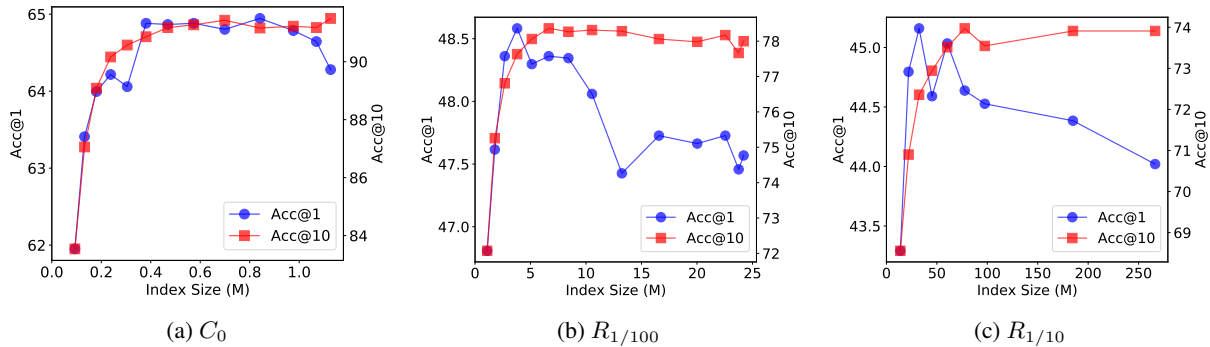
Figure 2: The trade-off between the index size and validation retrieval accuracy by changing filter thresholds on random subcorpora with different sizes, (a) C_0 , (b) R_{1/100} , and (c) R_{1/10} . A threshold that gives better accuracy with a smaller index size exists. Acc@1 (blue) is more unstable than Acc@10 (red). Interestingly, the index size of peak EM@1 is smaller than that of peak Acc@10.
