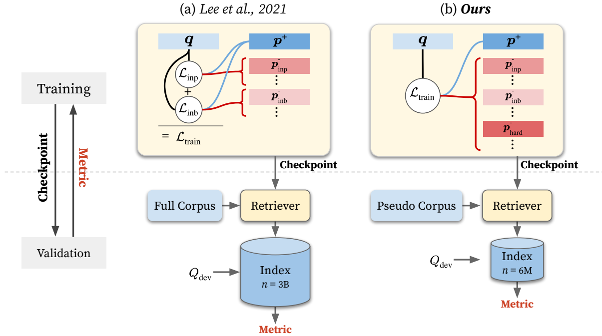
Figure 1: Comparison of the (a) original (Lee et al., 2021a) and (b) proposed procedure for DensePhrases training (top) and validation (bottom). We unify training loss terms \mathcal{L}_{inp} and \mathcal{L}_{inb} that enforce the representation of a question ( q ) similar to the representation of a positive phrase ( p^+ ) while contrasting from representations of in-passage negative phrases ( p_{inp}^- ) and in-batch negative phrases ( p_{inb}^- ) respectively into a single term \mathcal{L}_{train} and expand negatives in number and difficulty with hard negatives ( p_{hard}^- ). Also, we use a retrieval accuracy on the development set Q_{dev} using a smaller corpus instead of the full corpus as an efficient validation metric for selecting the best checkpoint. Query-side fine-tuning and token filtering are not described in this overview figure.
