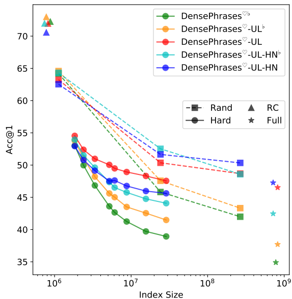
Figure 3: Validation results on open-domain QA. We plot retrieval accuracy (Acc@1) on indexes with different sizes (log-scale) from random and hard subcorpora. Random subcorpora (■) starts with C_0 and is extended to R_{1/100} and R_{1/10} . Hard subcorpora (●) include H_k for k \in \{1, 2, 4, 8, 10, 16, 32, 64\} . We also plot reading comprehension (RC) accuracy 8 and retrieval accuracy on the full index with filtering. We compare five different models with or without our proposed training methods and query-side fine-tuning. All models are trained and evaluated on Natural Questions. UL, HN, and b indicate a model trained with the unified loss, hard negatives, and before query-side fine-tuning.
