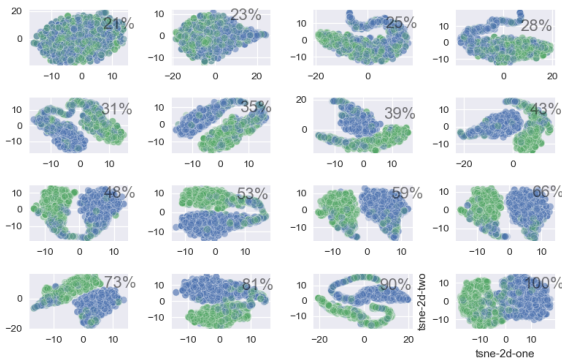
Figure 8: Class Separability Between Class Representations At Each Iterative Pruning Step on PAWSX.
