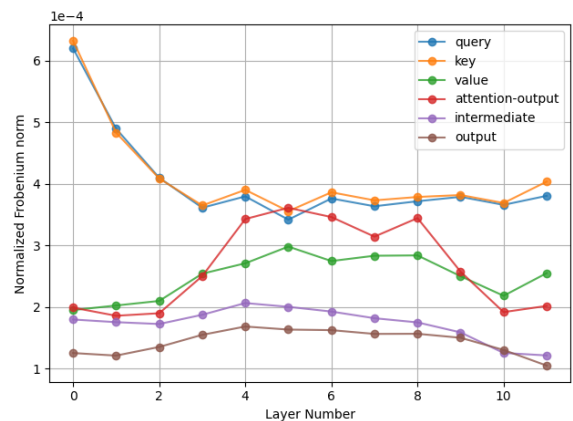
Figure 7: Pruned Model Weight Norms Per Layer
