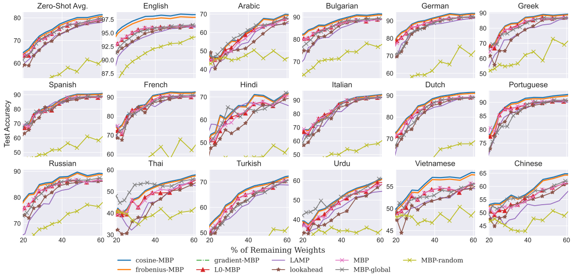
Figure 4: Part of Speech Tagging Test Accuracy.
