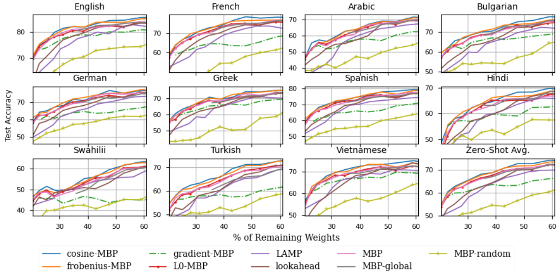
Figure 6: Zero-Shot XNLI Results Per Language After Iteratively Fine-Pruning XLM-RoBERTa Base
