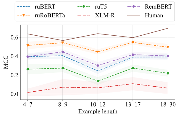
Figure 2: Results on the RuCoLA test set grouped by five quintiles of the sentence length.
