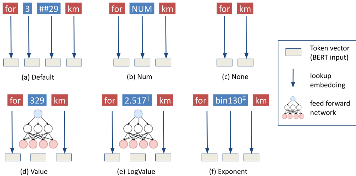
Figure 1: Different number encoders as described in Section 2. † 2.517 is \log_{10} 329 . ‡ 329 collapses to the 130 th bin out of 200 log-scaled bins within our range of [1e - 4, 1e + 6] .
