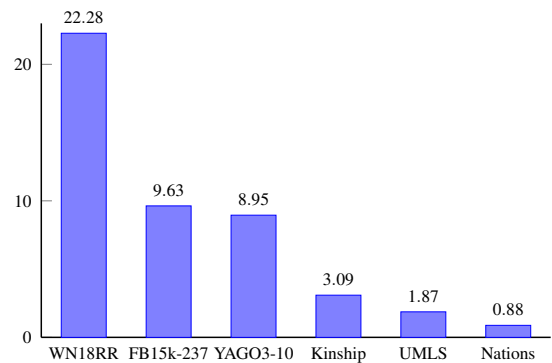
Figure 2: KL divergence of p_d(y|x) between training and test relations for each dataset
