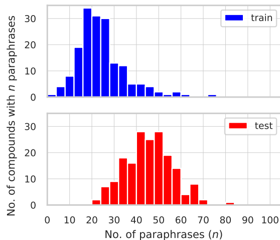
Figure 2: Distribution of paraphrase count in train and test part of SemEval-2013 Task-4 datasets.
