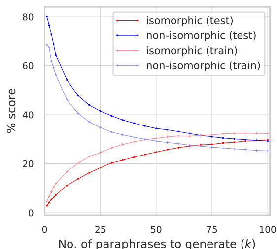
Figure 3: Performance of T5-based system for different value of k (number of paraphrases to generate) on train and test sets of SemEval-2013 Task-9 dataset.
