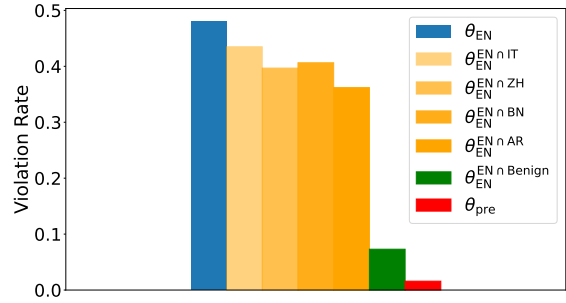
Figure 3: Qwen2-7B violation rates on the English language split of MultiJail after fine-tuning attack (blue) using English harmful data, stitching the bilingual intersection safety parameters localized by SIL (orange bars), benign datasets (green), and its original violation rate (red). gauges may influence the reported violation rates; Second, linguistic characteristics, such as sentence structure, vary significantly between different languages, thus affecting how well the safety capabilities generalize from one language to another.
