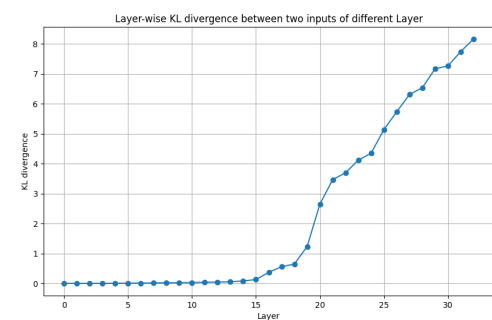
(b) Hallucination
