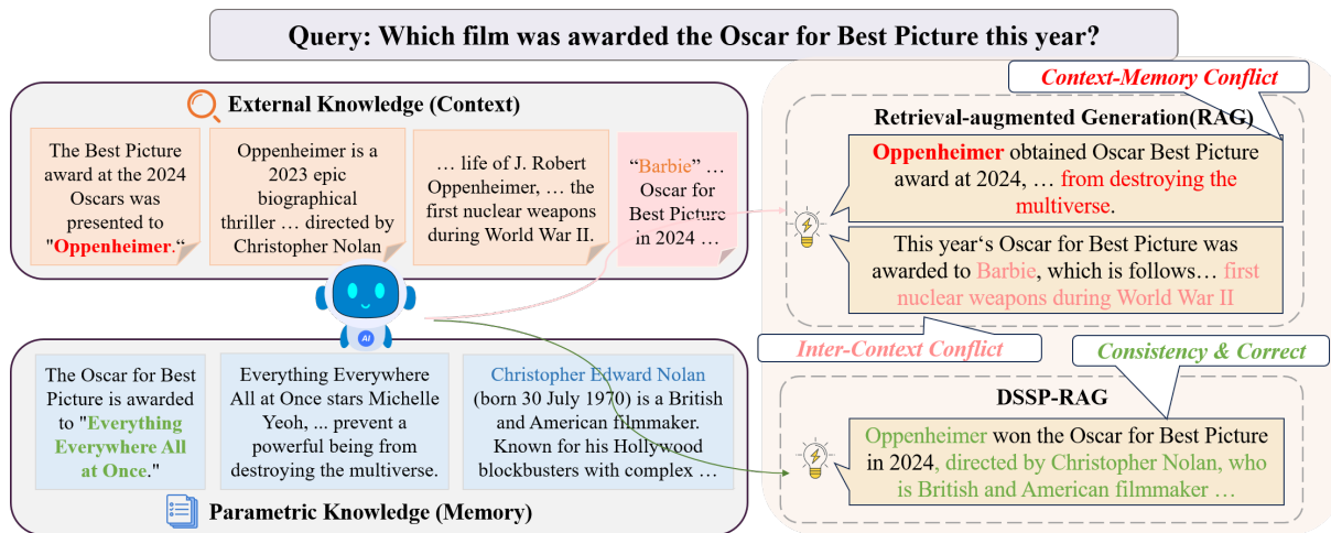
Figure 1: Comparison of Inference Results Using External vs. Parameterized Knowledge Across Methods
